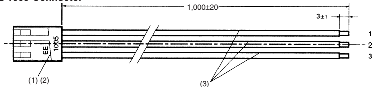
EE-1005 Connector
